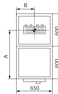
Depth: 1200 mm
