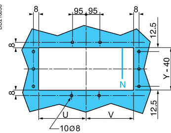
1000 to 5000 A
